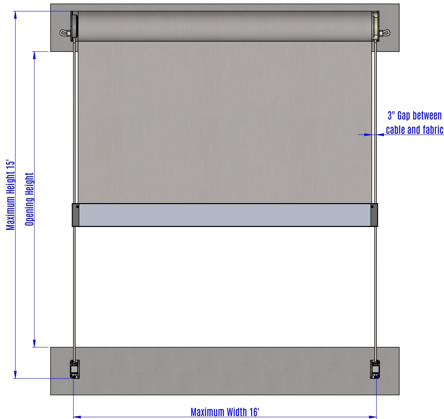
FRONT VIEW
