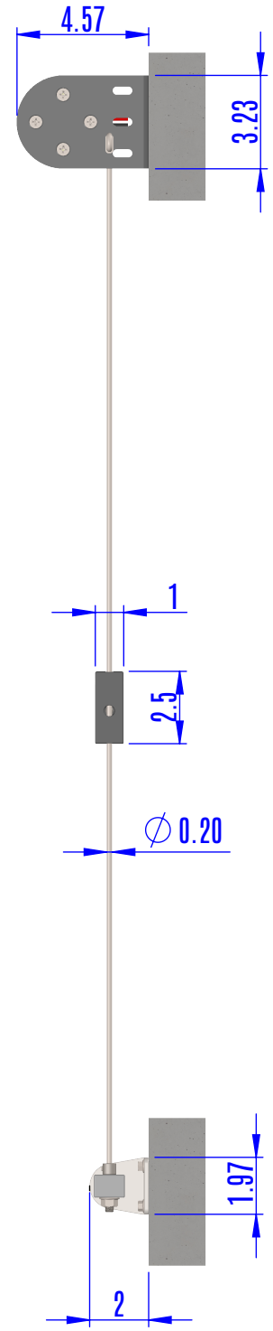
SIDE VIEW
